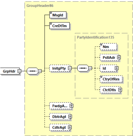
Abbildung 87: pain.002.001.10, Group Header
