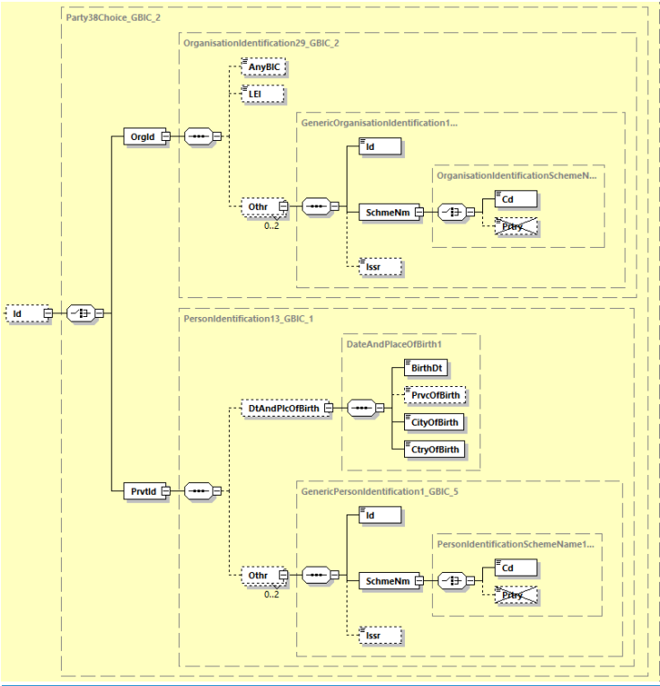
Abbildung 81: pain.001.001.09, Identification
