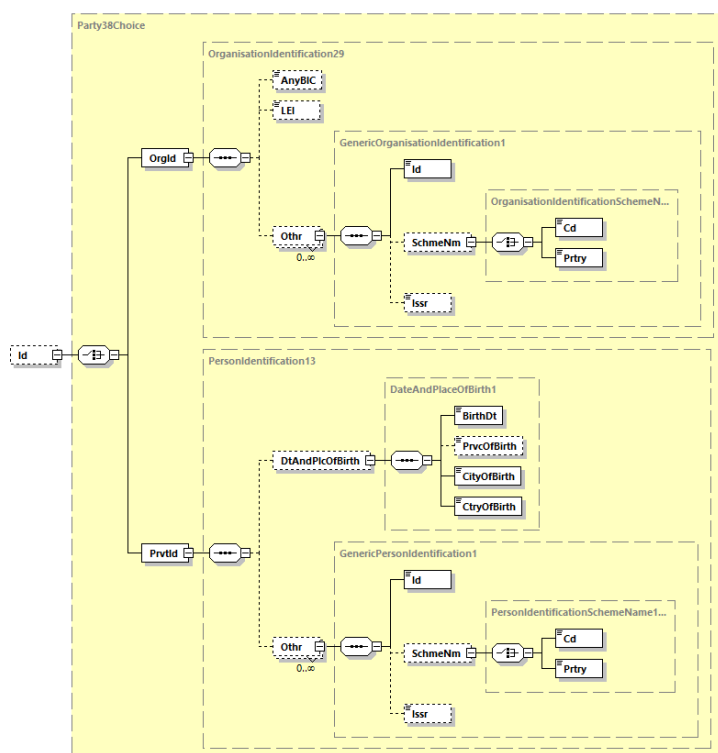
Abbildung 97: pain.002.001.10, Identification
