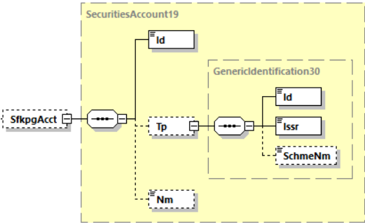
Abbildung 121: camt.053.001.08, SfkpgAcct
