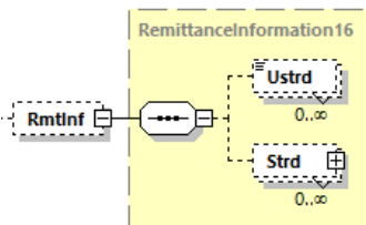
Abbildung 52: pain.002.001.10, Remittance Information
