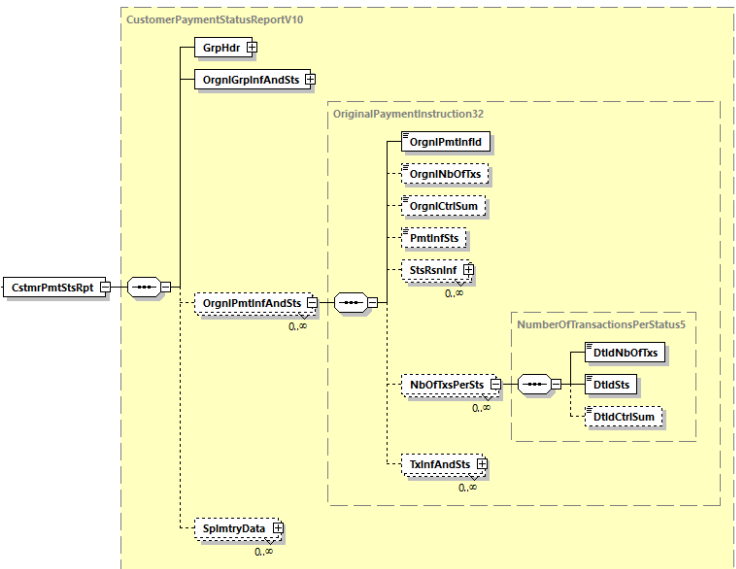
Abbildung 45: pain.002.001.10, Customer Payment Status Report
