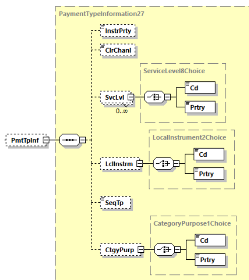
Abbildung 94: pain.002.001.10, Payment Type Information
