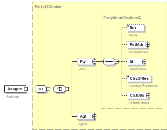
Abbildung 156: camt.029.001.06, Assgne
