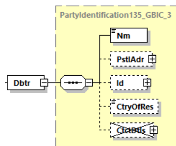
Abbildung 75: pain.001.001.09, Debtor
