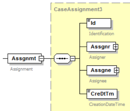
Abbildung 154: camt.029.001.06, Assgnmnt
