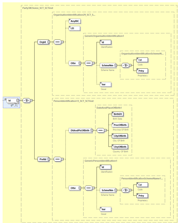
Abbildung 30: pain.001.001.09, Identification
