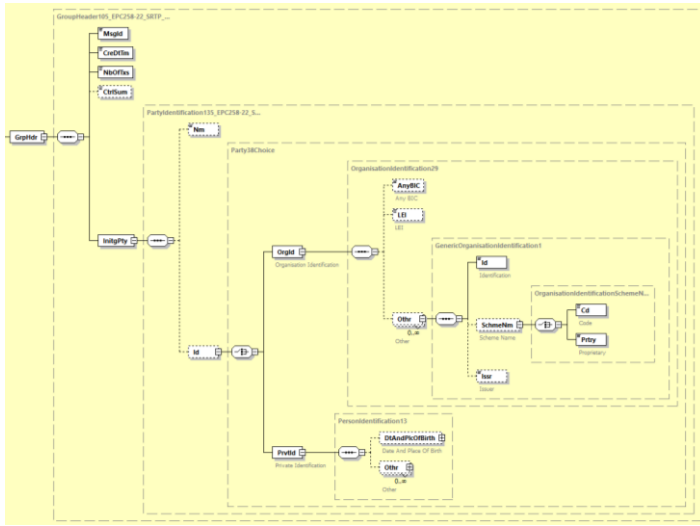
Abbildung 3: pain.013.001.10, Group Header
