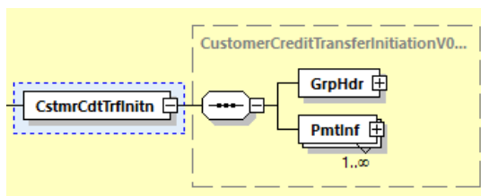
Abbildung 23 pain.001.001.09: Customer Credit Transfer Initiation
