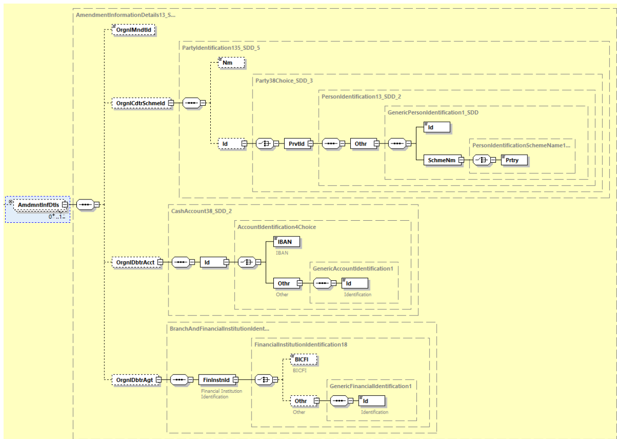
Abbildung 39: pain.008.001.08, Amendment Information Details
