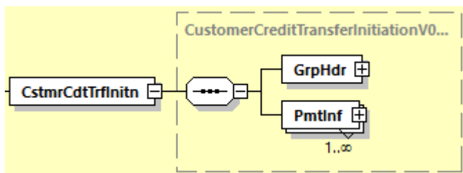
Abbildung 140 pain.001.001.09: Customer Credit Transfer Initiation
