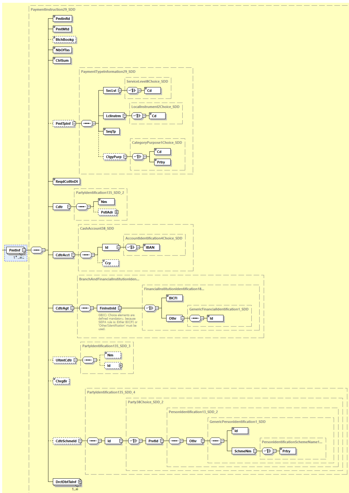
Abbildung 36: pain.008.001.08, Payment Information
