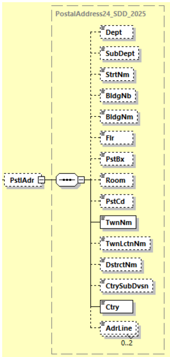
Abbildung 41: pain.008.001.08, Postal Address
