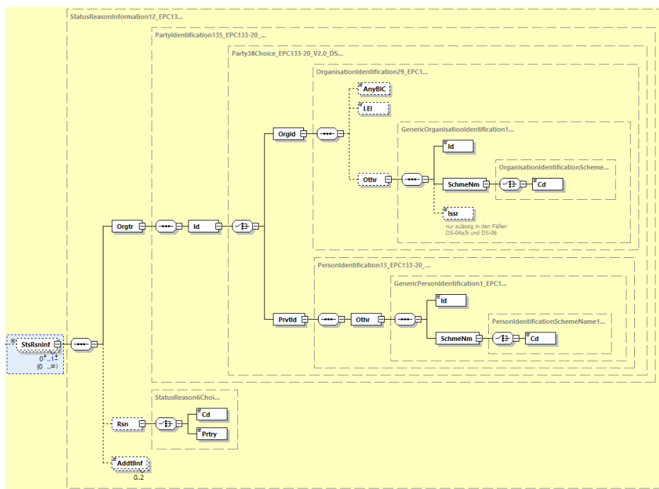
Abbildung 12: pain.014.001.07, Status Reason Information
