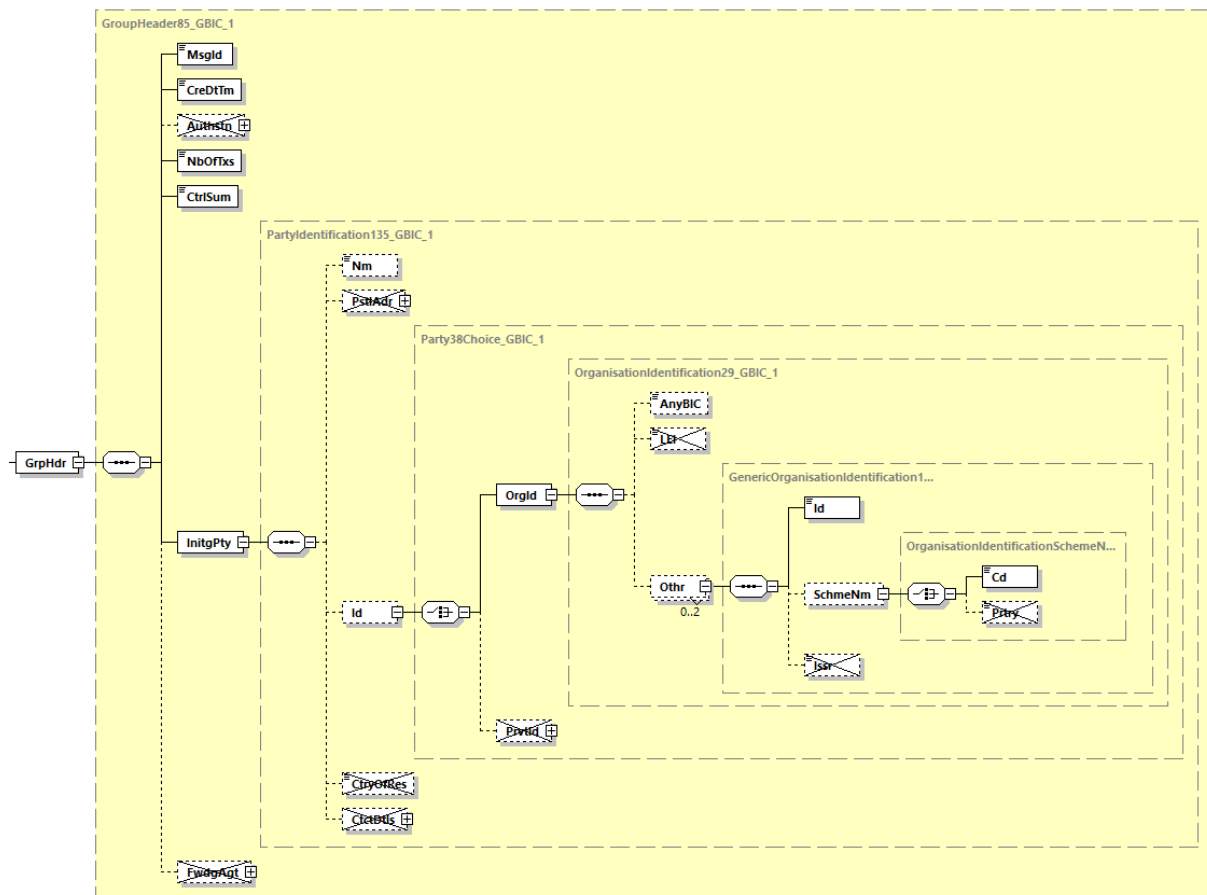
Abbildung 73: pain.001.001.09, Group Header
