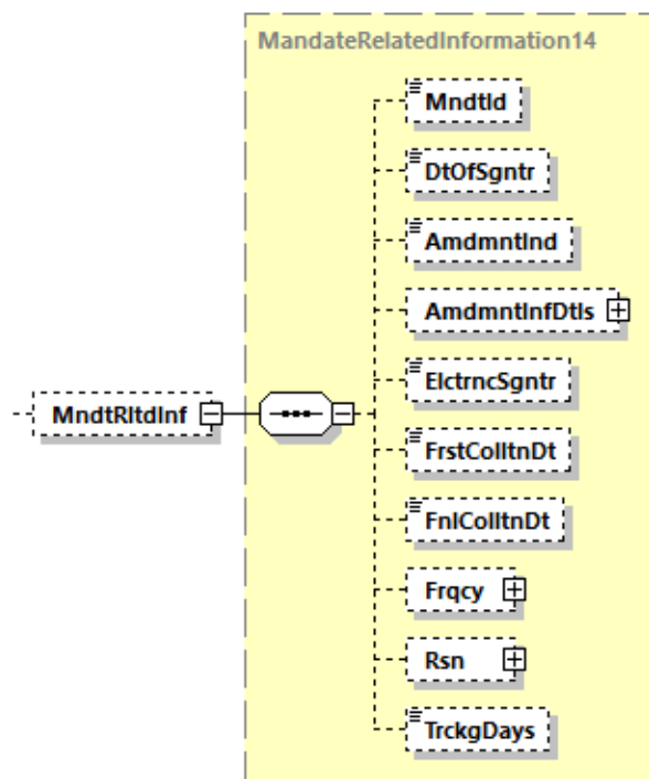
Abbildung 51: pain.002.001.10, Mandate Related Information
