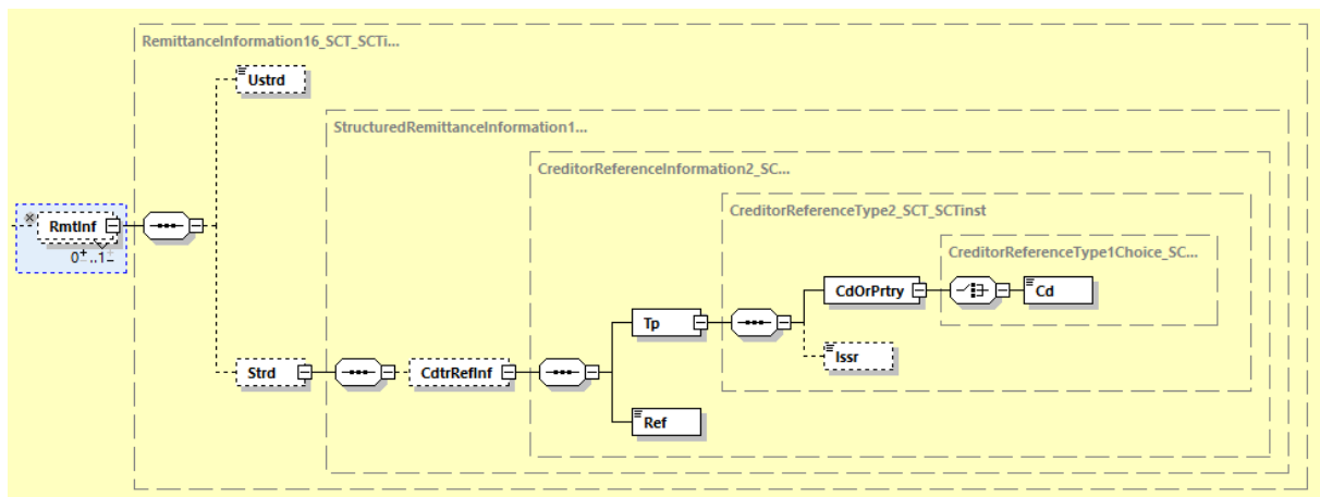
Abbildung 145: pain.001.001.09, Remittance Information
