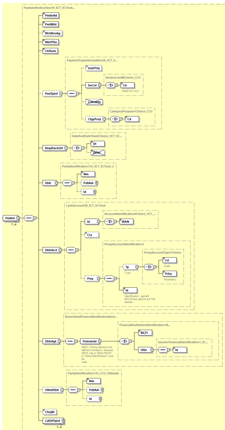
Abbildung 143: pain.001.001.09, Payment Information
