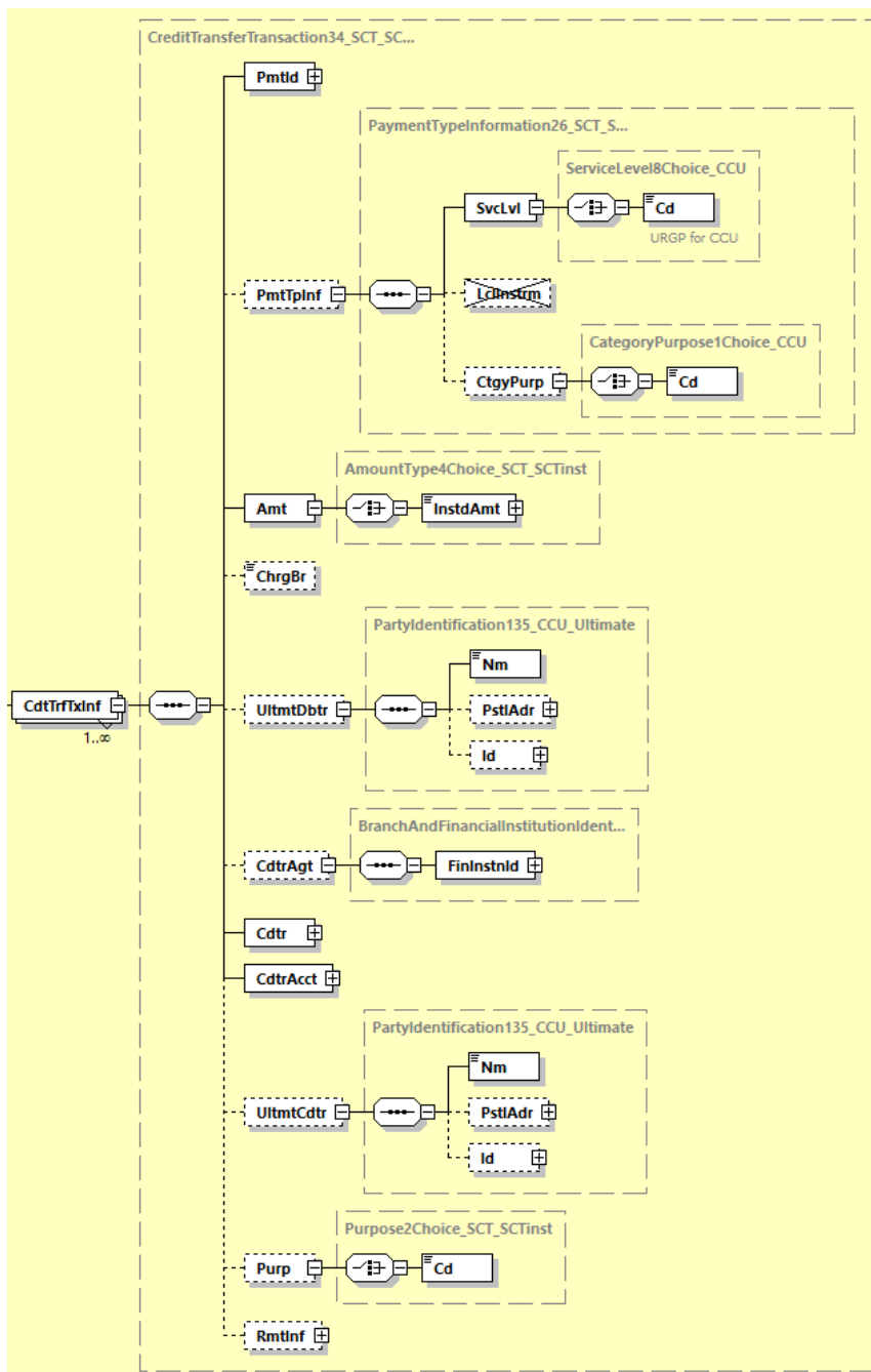
Abbildung 144: pain.001.001.09, Credit Transfer Transaction Information
