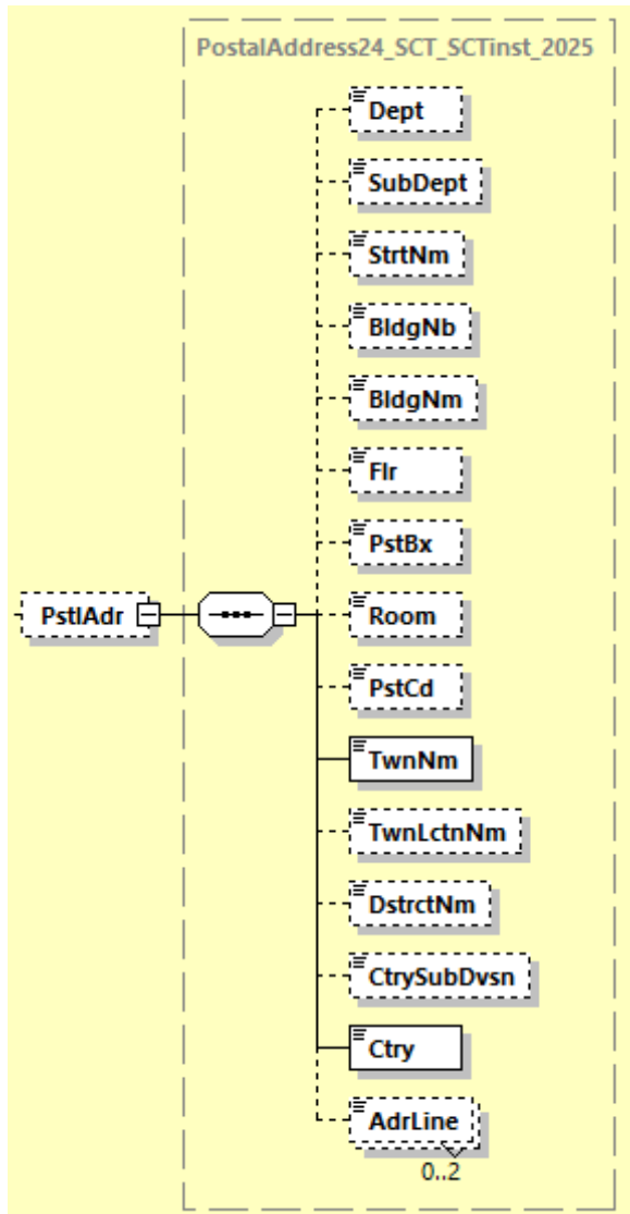
Abbildung 146: pain.001.001.09, Postal Address
