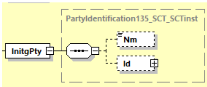
Abbildung 142: pain.001.001.09, Initiating Party
