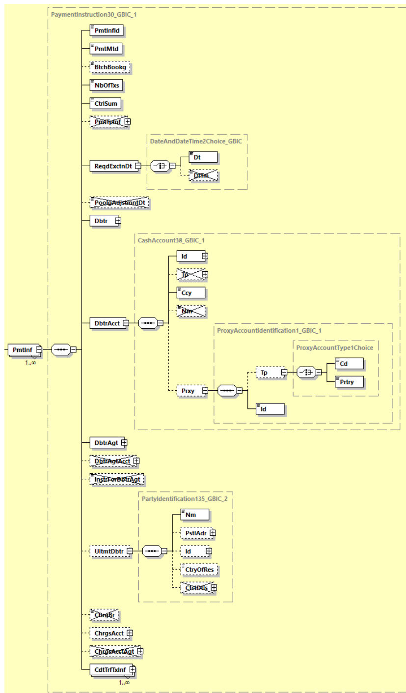
Abbildung 74: pain.001.001.09, Payment Information
