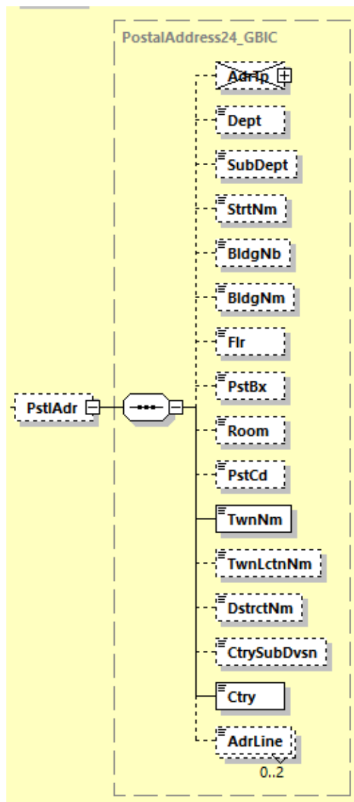
Abbildung 81: pain.001.001.09, Postal Address
