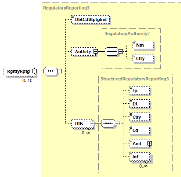
Abbildung 78: pain.001.001.09, Regulatory Reporting
