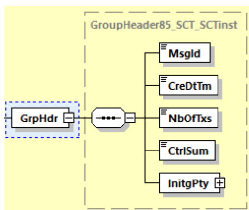
Abbildung 141: pain.001.001.09, Group Header
