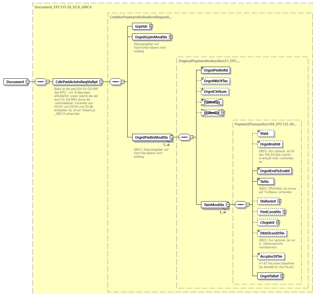
Abbildung 8: pain.014.001.07, Creditor Payment Activation Request Status Report
